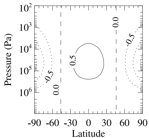
Figure 2. Latitude-height cross section of the deviation of the prescribed thermal relaxation field from the global mean in Figure 1. Calculated from T_H(\eta)\cos\phi in section 2 and Table 1.
